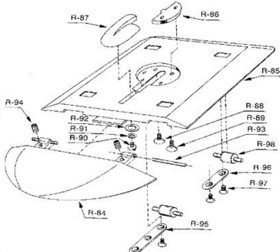
STANDARD ASSEMBLY
