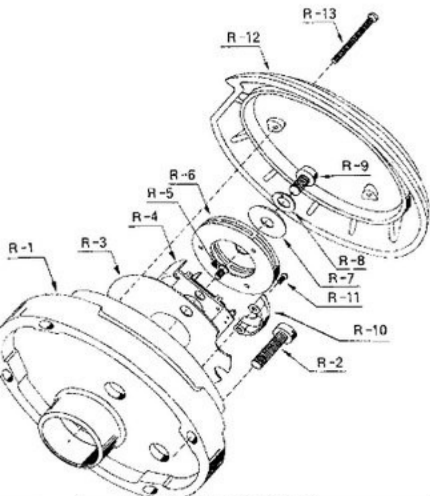
SHARPENING ASSEMBLY
