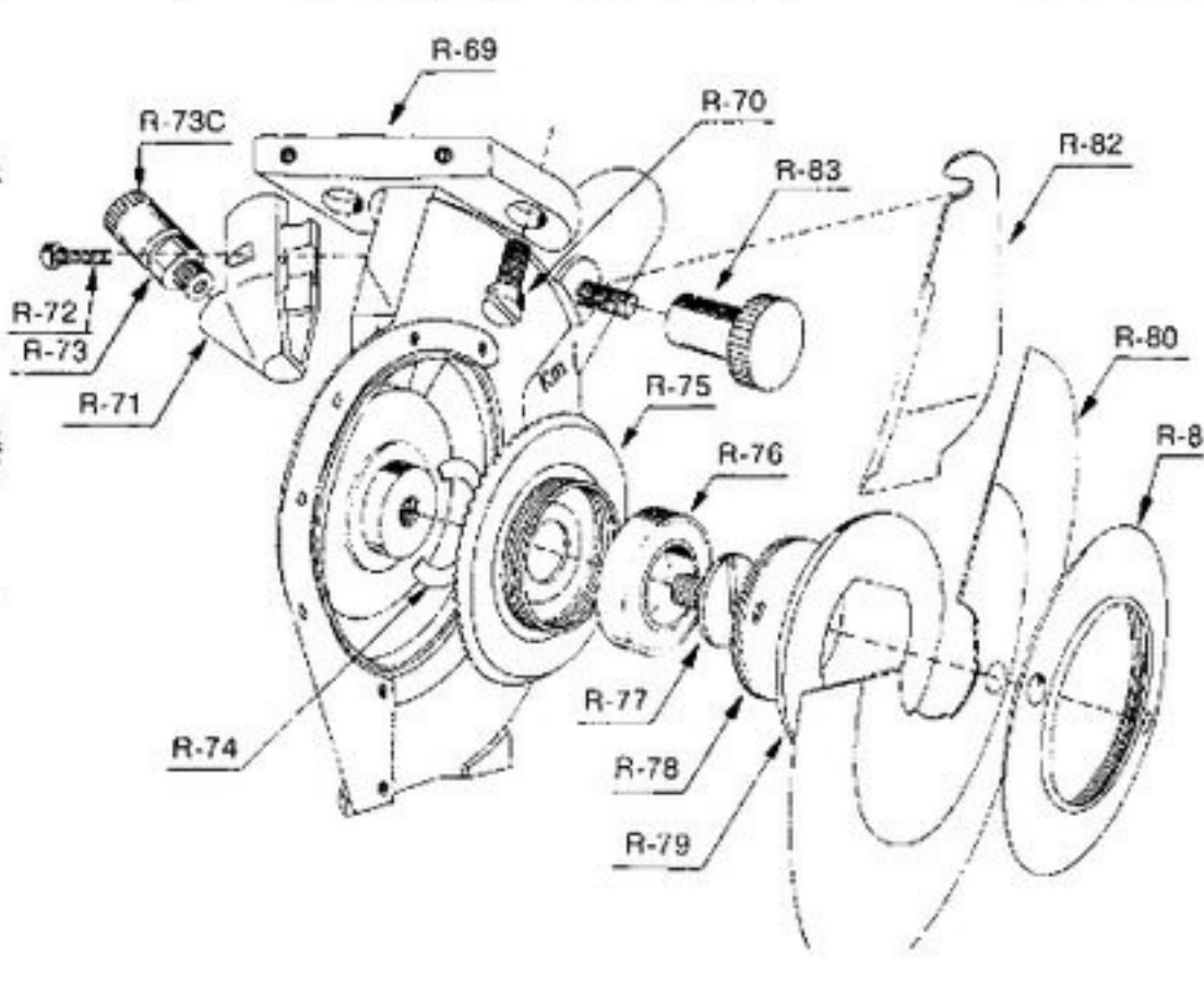
STANDARD ASSEMBLY
