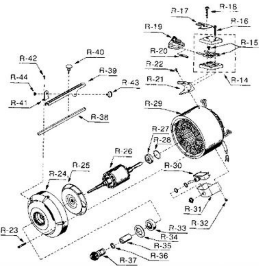
REAR BEARING HOUSING ASSEMBLY
