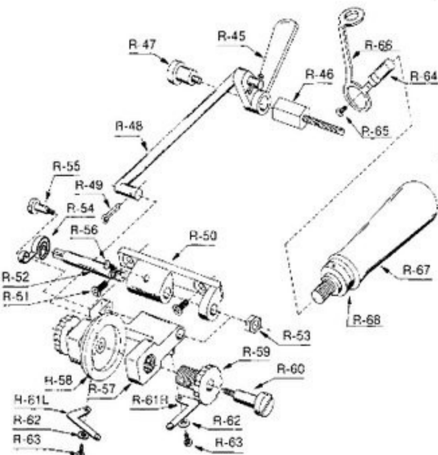
SHARPENING ASSEMBLY
